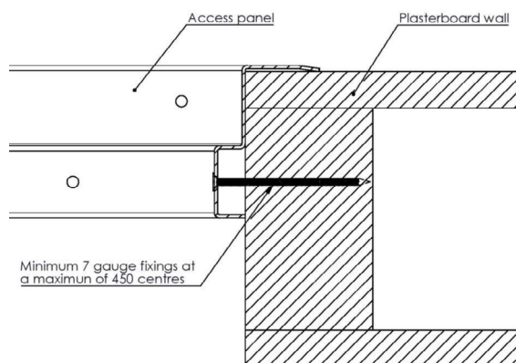
PLASTERBOARD Install Profile
