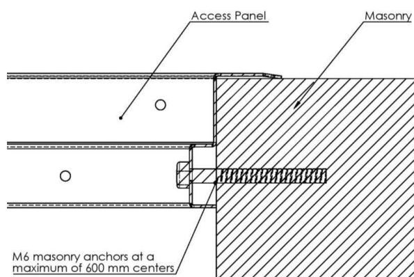
MASONRY Install Profile
