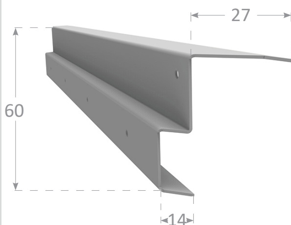
Frame Type FLANGED EDGE (FEATHERED EDGE)
